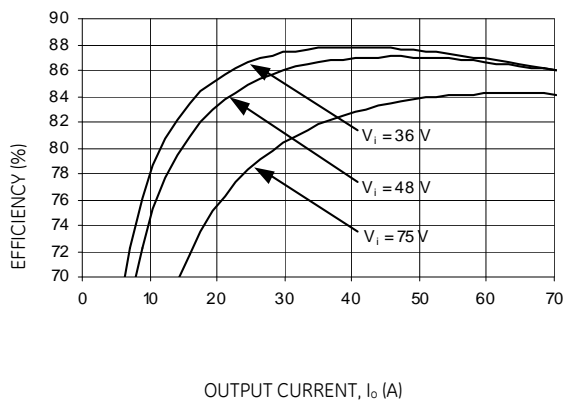
Figure 32. Converter Efficiency Vs Load at Room temperature.
