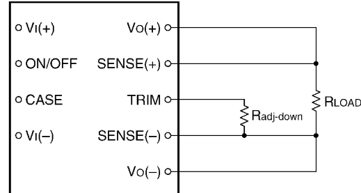
Figure 48. Circuit Configuration to Decrease Output Voltage.
