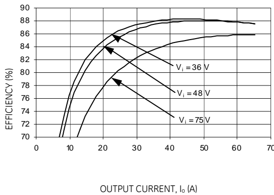
Figure 26. Converter Efficiency Vs Load at Room temperature.
