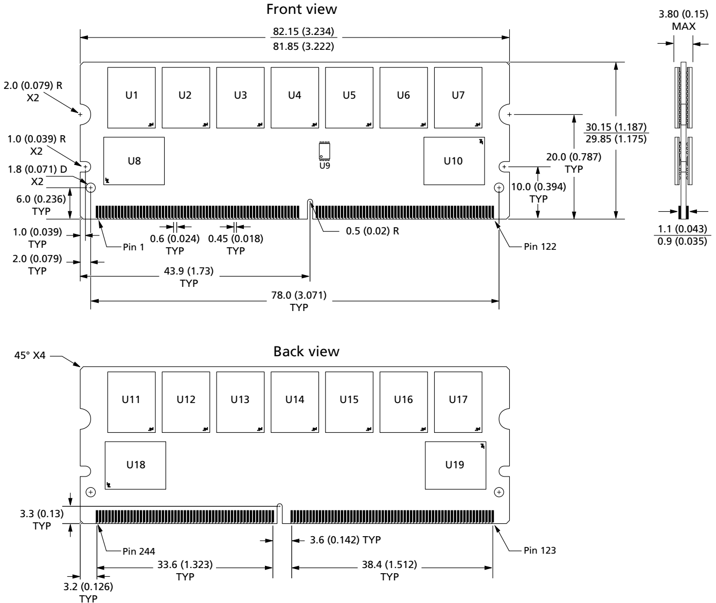
Figure 3: 244-Pin DDR3 Mini-UDIMM (MO-244)
