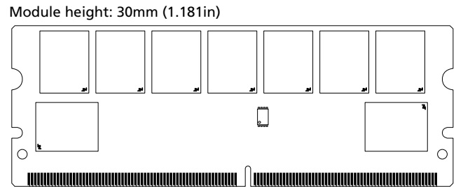
Figure 1: 244-Pin Mini-UDIMM (MO-244, R/C B)
