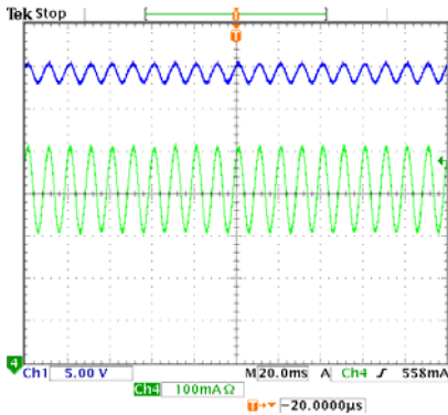
Figure 20. 90Vac, Full load Channel 1: Vout, 5V/Div Channel 4: Iout, 100mA/Div
