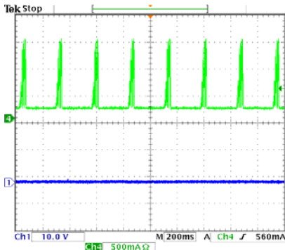
Figure 22. 90Vac, Full load Channel 1: Vout, 10V/Div Channel 4: Iout, 500mA/Div
