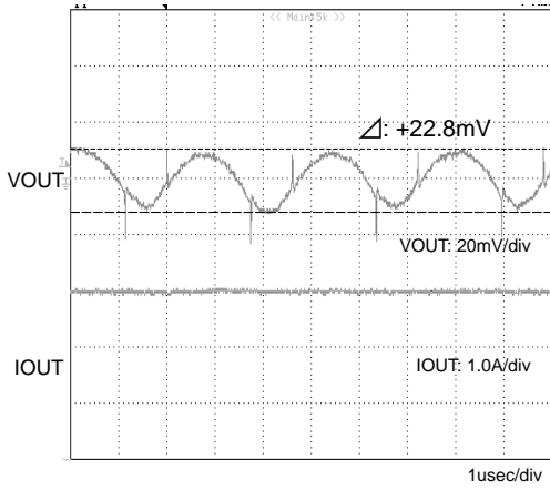
Fig.16 Output Ripple Voltage (VIN= 12V VOUT= 3.3V L= 10μH Cout =22μF Iout= 3.0A)
