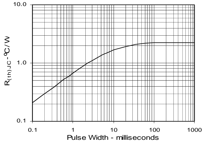
Fig. 13. Maximum Transient Thermal Resistance
